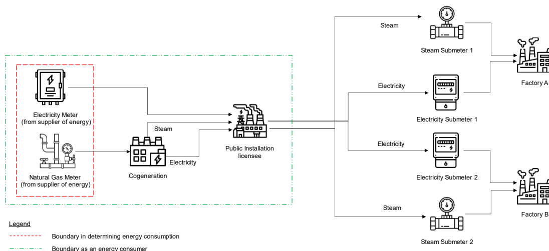
Figure 18: Public installation licensee with cogeneration.
