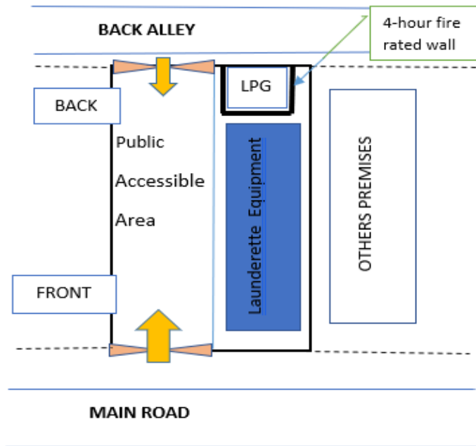
TYPE B- LPG STORAGE PLACED INSIDE OF LAUNDERETTE PREMISES
