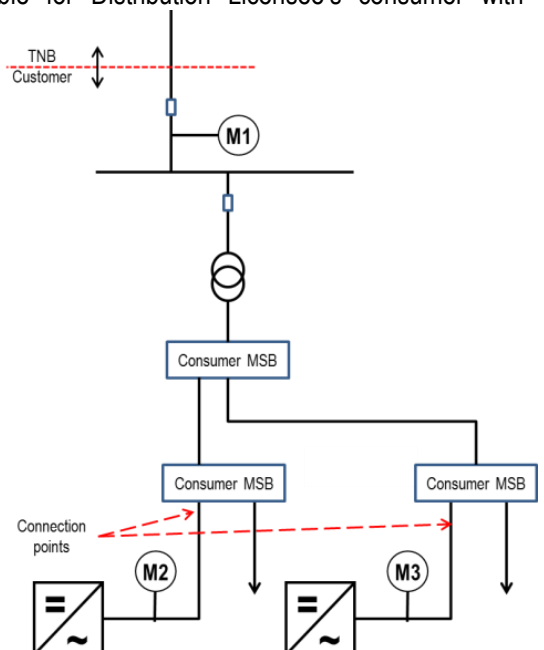
Fig. 5.4: Type B connection
